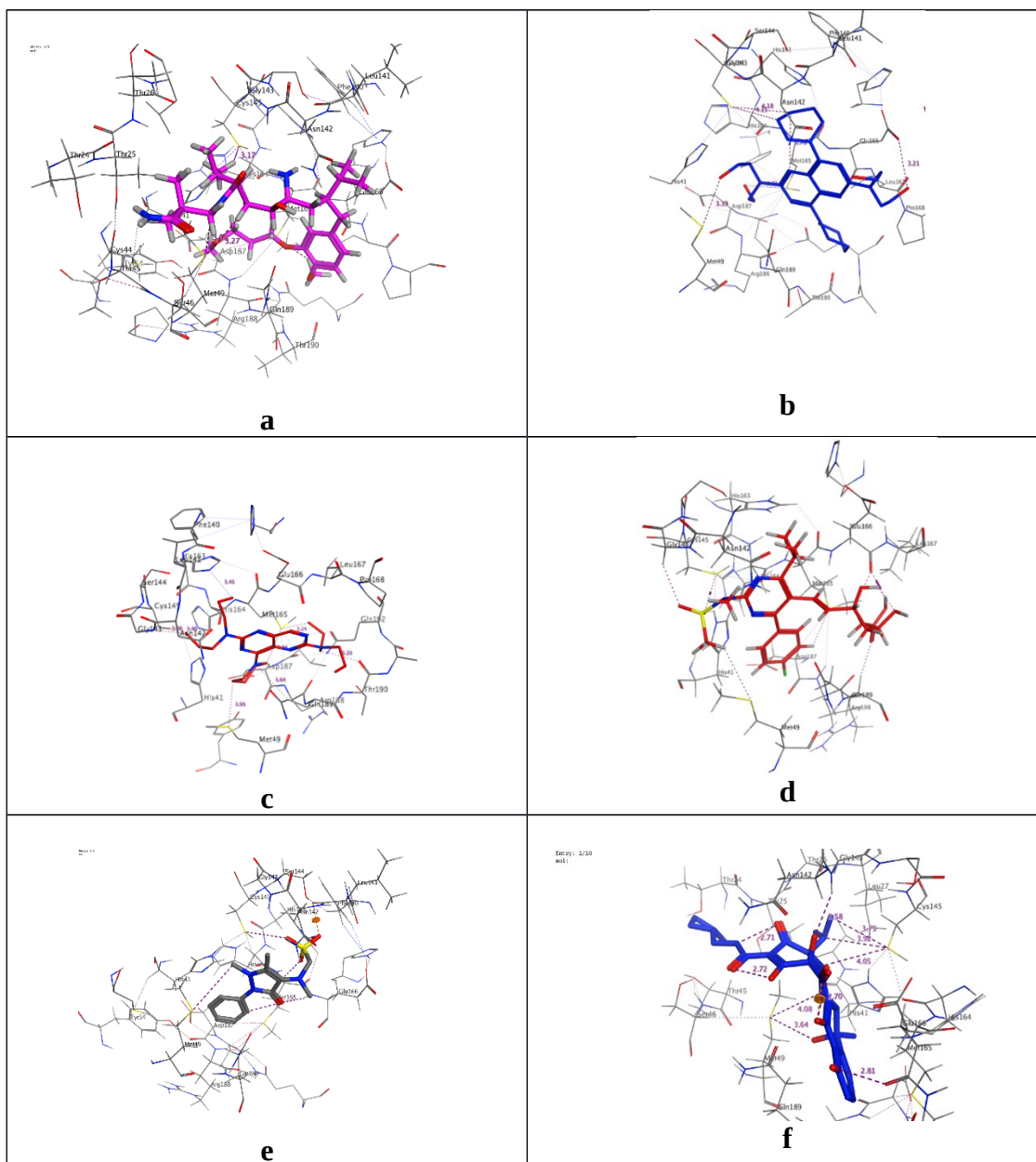
Fig. 2: 2D representation of docking of compounds: Aliskiren a , Dipyridamole b , mopidamol c , rosuvastatin d , metamizole e , rolitetracycline f , darunavir g , and N3 h into the N3 binding site in the COVID-19 protease. Aliskiren was showed the highest binding energy in comparison with the other compounds which showed nearly equal or moderately lesser binding energies.
