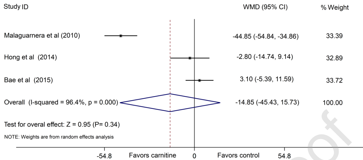
Figure 8 Forest plot of LDL-C change outcome
