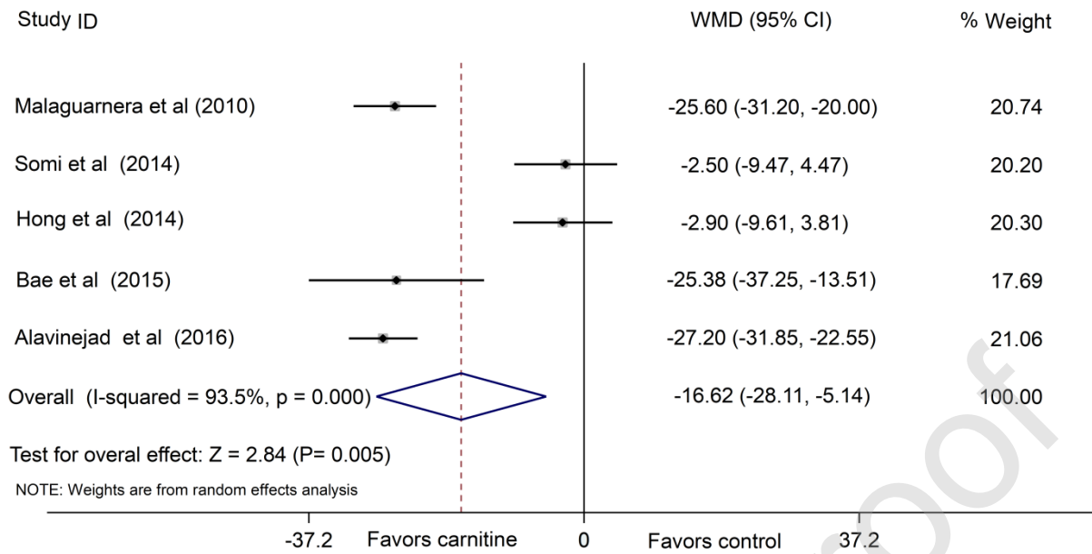
Figure 2 Forest plot of AST change outcome
