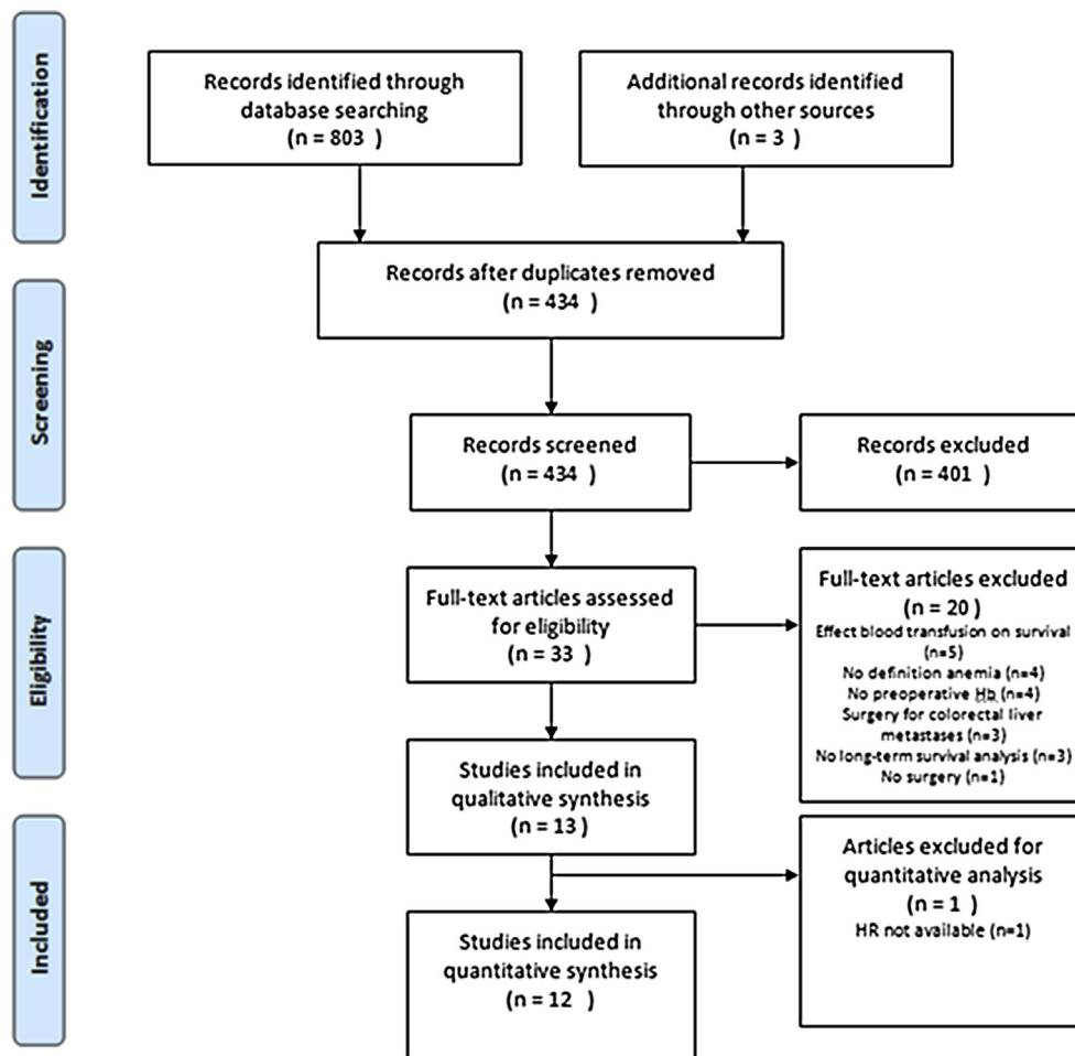
Fig. 1. PRISMA flowchart.
